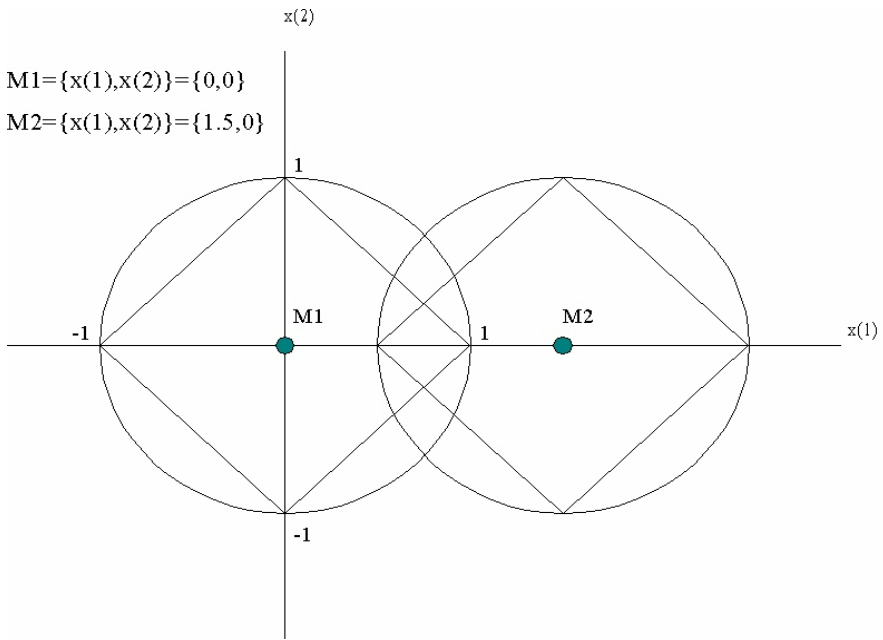
Figure 1: Illustration of the sets B_N(\mathbf{x}) and B_N^*(\mathbf{x}) as the basis for calculating the spherical covariance function E(m_N(0,0)m_N(1.5,0)) - given by the intersection of the unit circles - and the L_1 norm covariance function E(m_N^*(0,0)m_N^*(1.5,0)) - given by the intersection of the two othogons.
