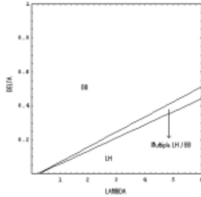
Figure 3: \gamma_n = 1/3 , r = 0.02 , (f_u, f_{lh}, f_{hh}) = (.3, .5, .9)
