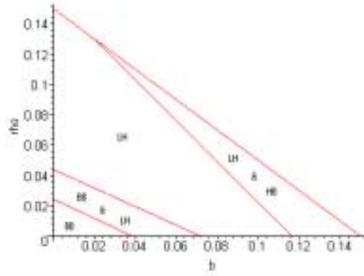
Figure 2: \gamma_n = 1/3 , r = .02 , (f_u, f_{lh}, f_{hh}) = (.3, .5, .9) , \lambda = 6 , \delta = .6
