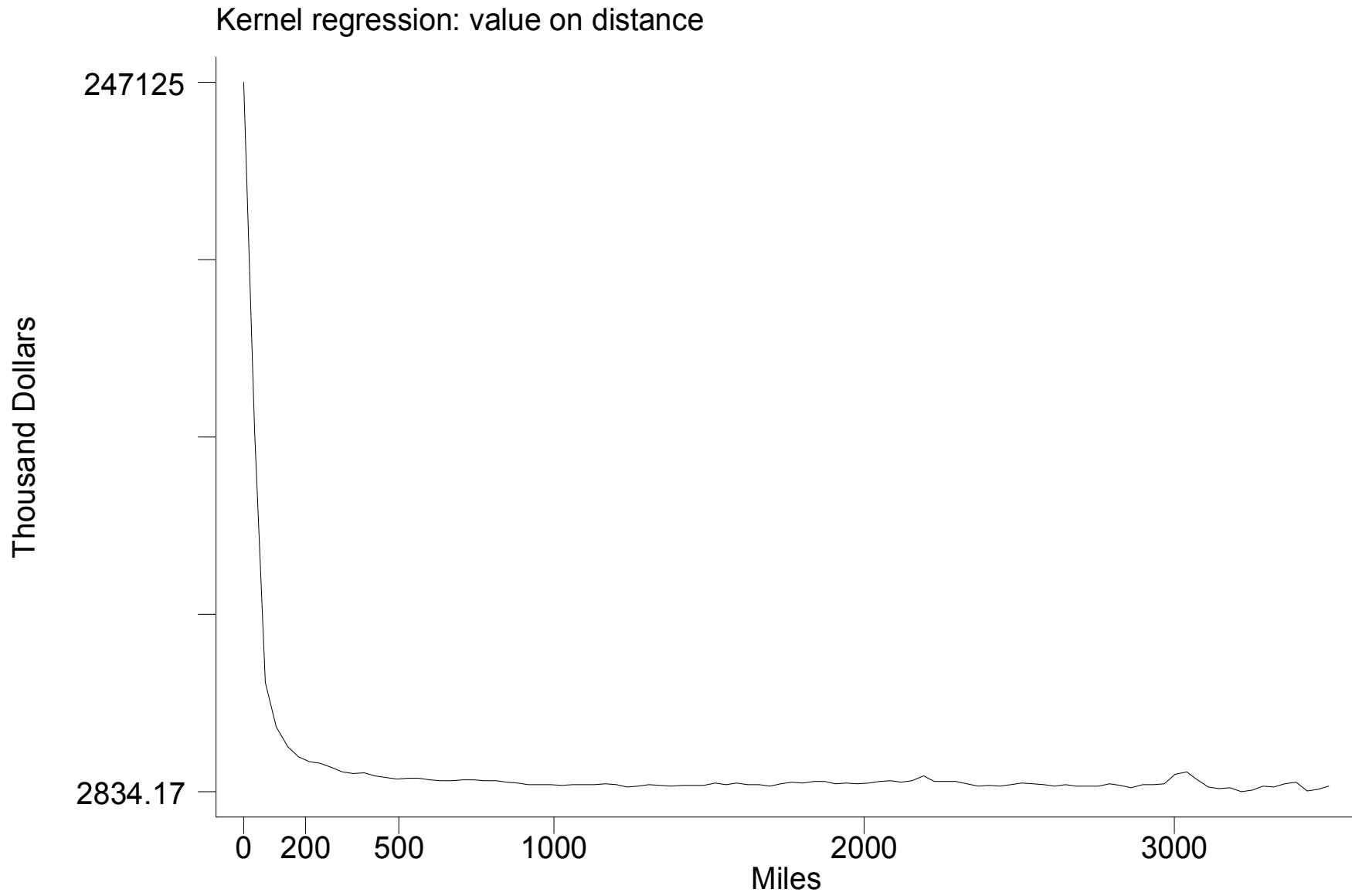
Figure 1: Kernel Regressions
